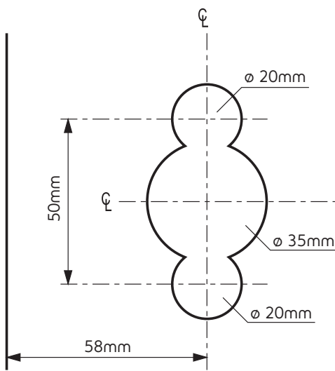
Lock cut out detail
