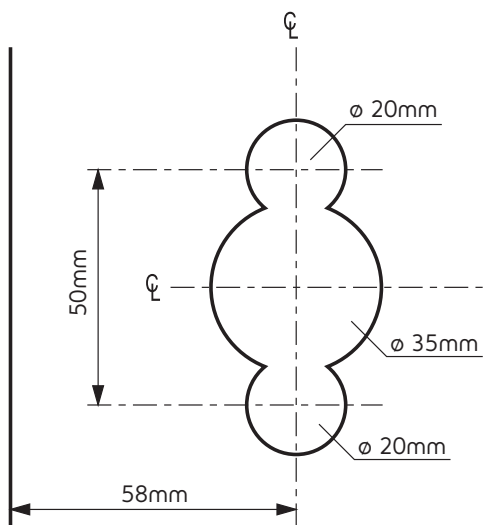
Lock cut out detail
