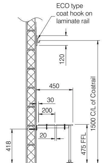
Section of Wall & Floor Mounted Seating
