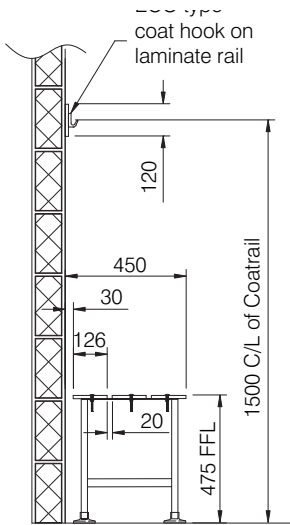
Section of Marathon Floor Mounted Seating
