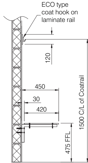
Section of Cantilevered Seating
