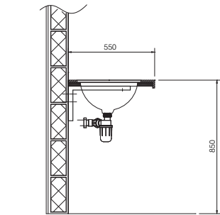
Side Section
